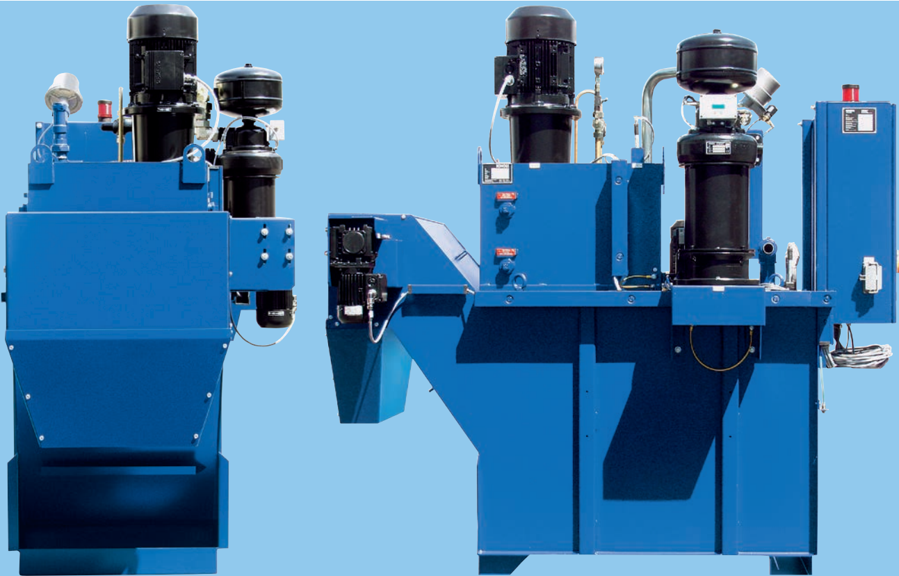
AF 5000 Tankinhalt 5000 l Tank capacity 5000 l
