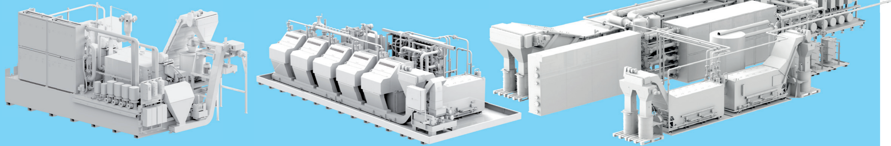
This filter system is designed for cleaning grinding oil in HSS/cast material processing. It contains four filter modules and their cleaning output is 1900 l/min.
