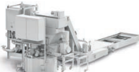
Conveyor with chip reducer, return pumping station RKR and pressure booster DHS
